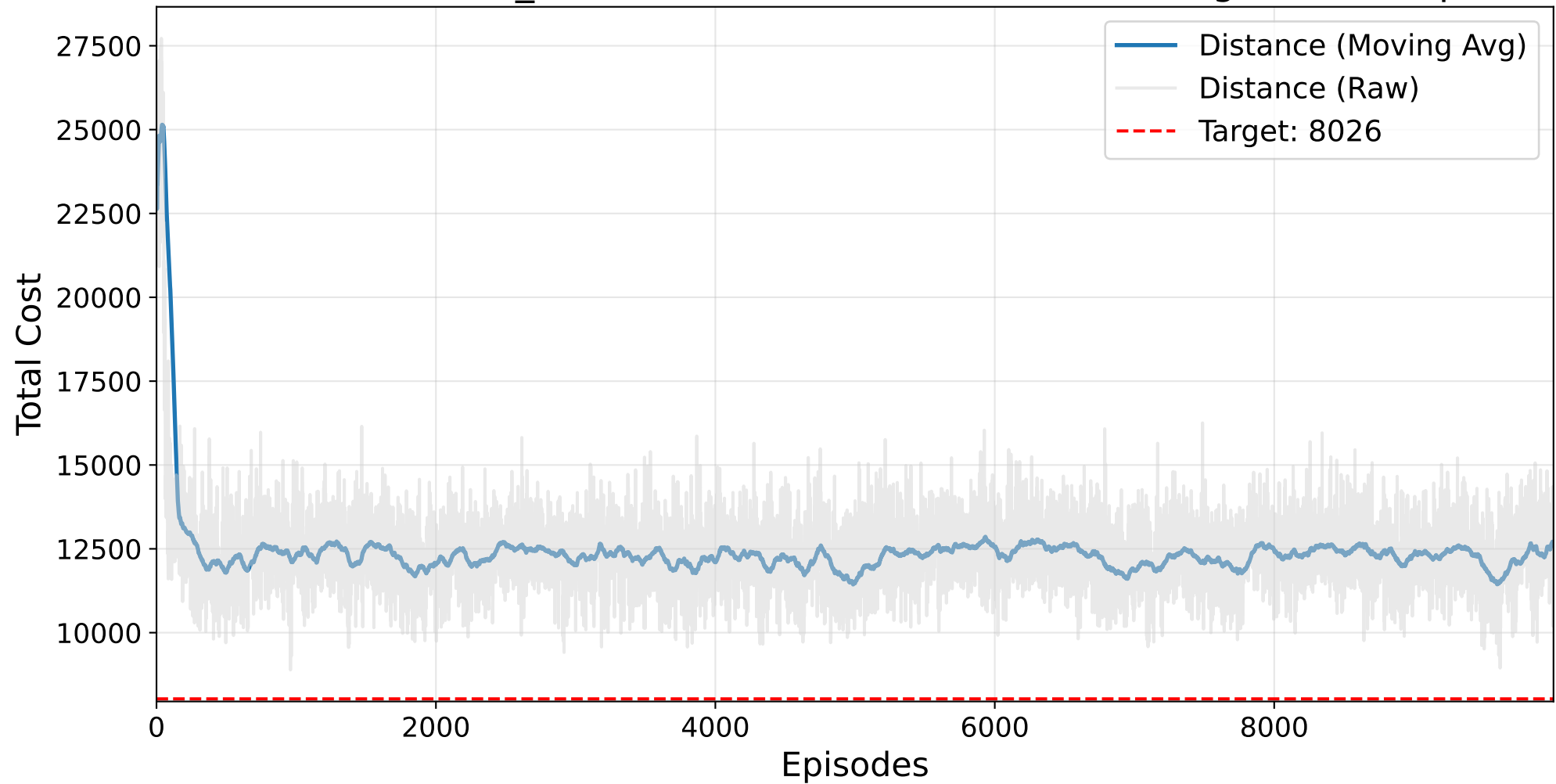
Final RANDOM_SEARCH Masked AutoRL-SOP Training - ft53.2.sop
